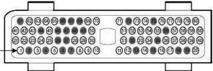
Front of the Allison Transmission Control Module Connector
